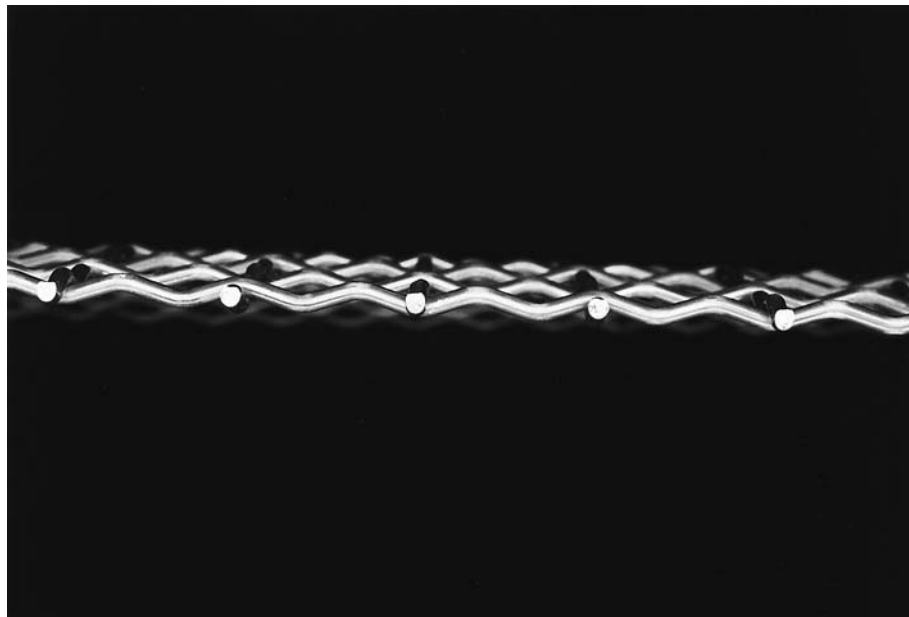
FIG. 7 Intermediate Crimp
