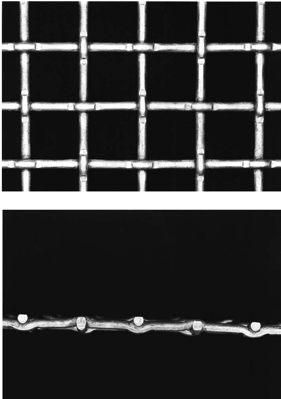
FIG. 8 Lock Crimp
